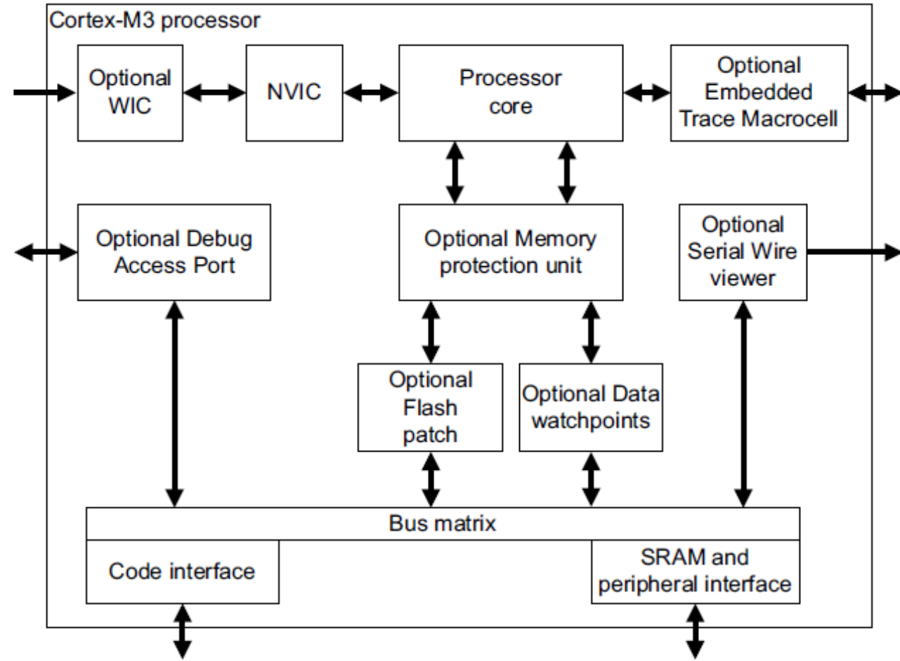
Figure 1-1 Cortex-M3 implementation
