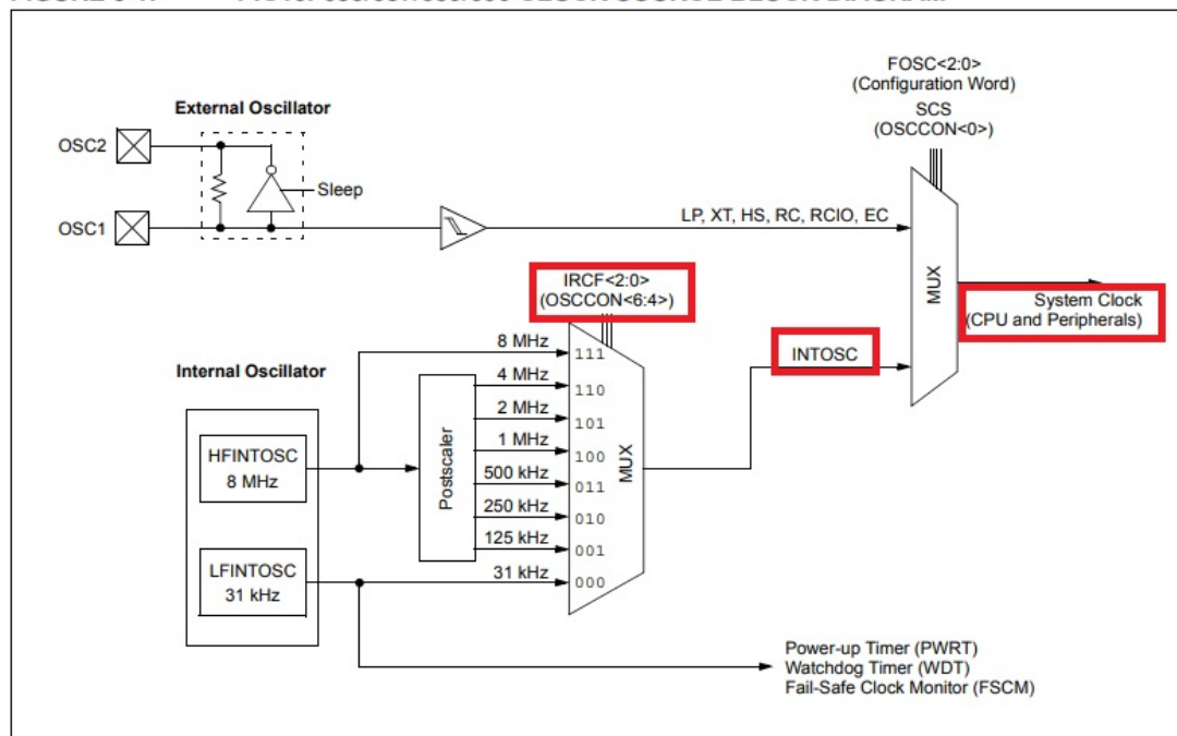
FIGURE 3-1: PIC16F685/687/689/690 CLOCK SOURCE BLOCK DIAGRAM
