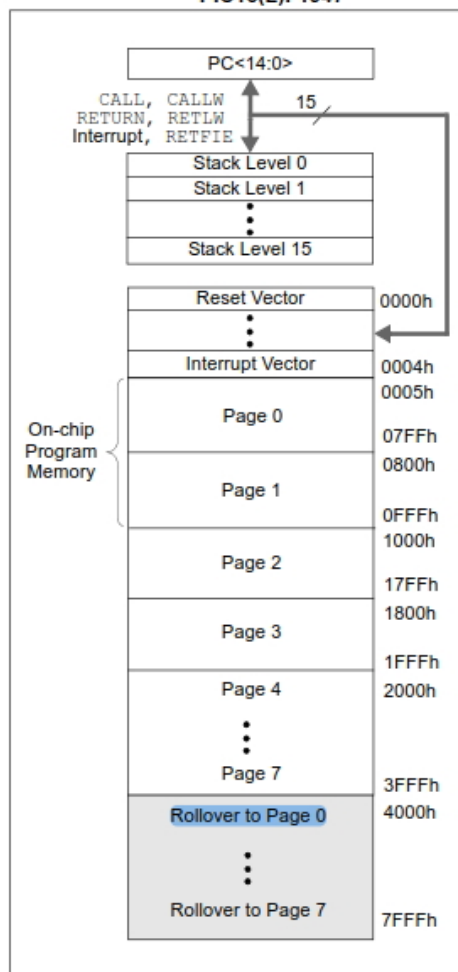
FIGURE 3-2: PROGRAM MEMORY MAP AND STACK FOR PIC16(L)F1947
