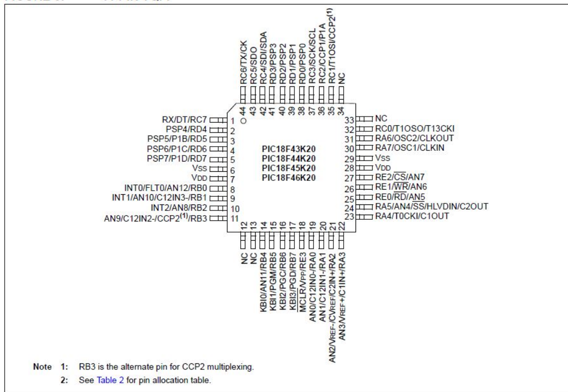
FIGURE 6: 44-PIN TQFP
