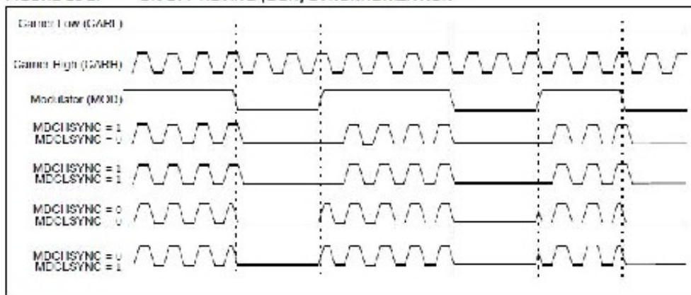
FIGURE 23-2: ON OFF KEYING (OOK) SYNCHRONIZATION
