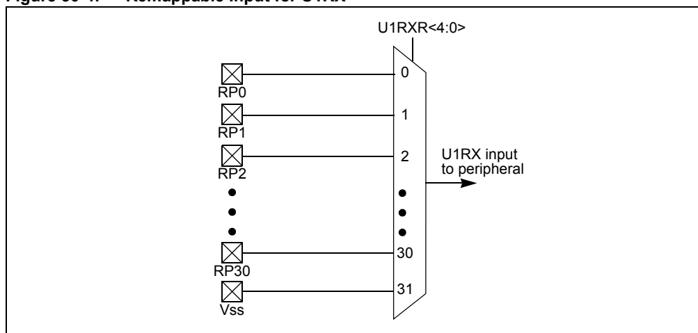
Figure 30-4: Remappable Input for U1RX
