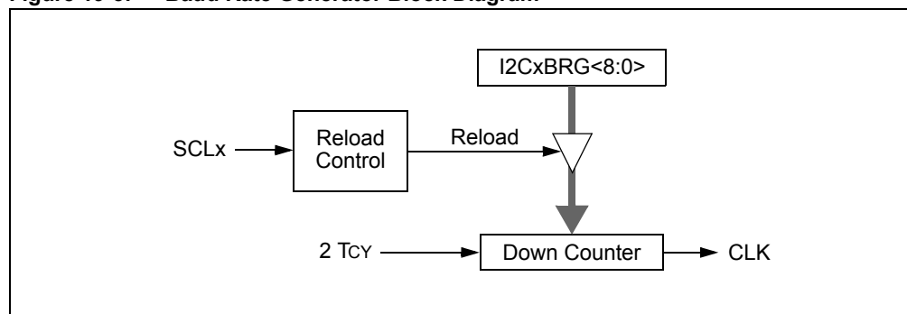
Figure 19-5: Baud Rate Generator Block Diagram
