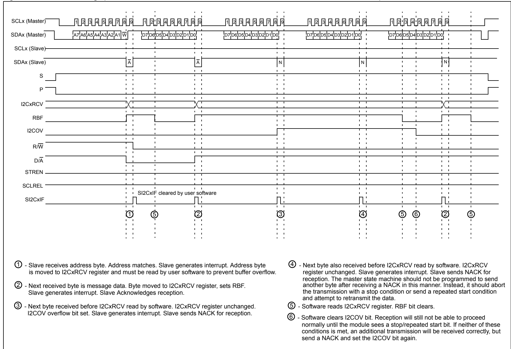
Figure 19-28: Slave Message (Write Data to Slave: 7-Bit Address; Buffer Overflow; A10M = 0; GCEN = 0; IPMIEN = 0)
