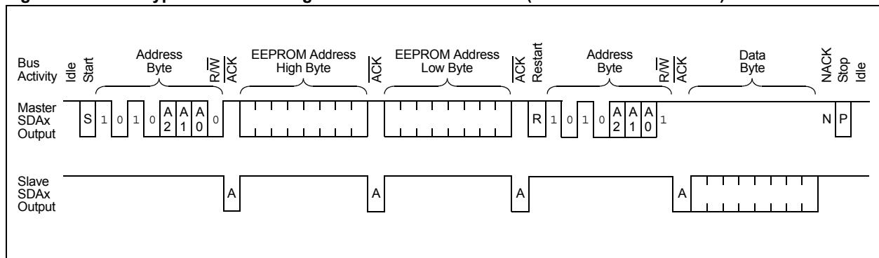
Figure 19-6: A Typical I 2 C™ Message: Read of Serial EEPROM (Random Address Mode)
