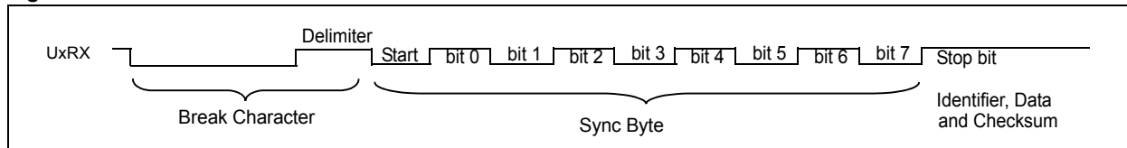
Figure 17-26: Frame Structure
