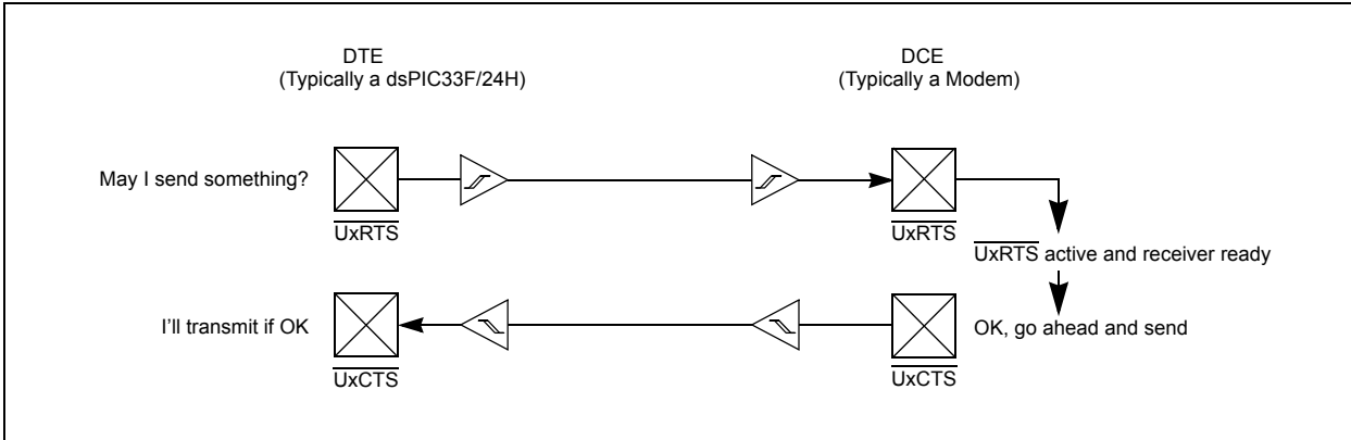
Figure 17-18: \overline{UxRTS}/\overline{UxCTS} Handshake for DTE-DCE (RTSMD = 1, Simplex Mode)
