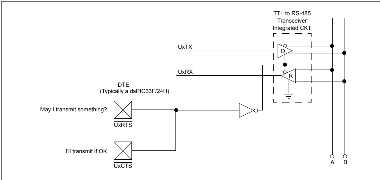
Figure 17-19: \overline{UxRTS}/\overline{UxCTS} Bus Enable for IEEE-485 Systems (RTSMD = 1)
