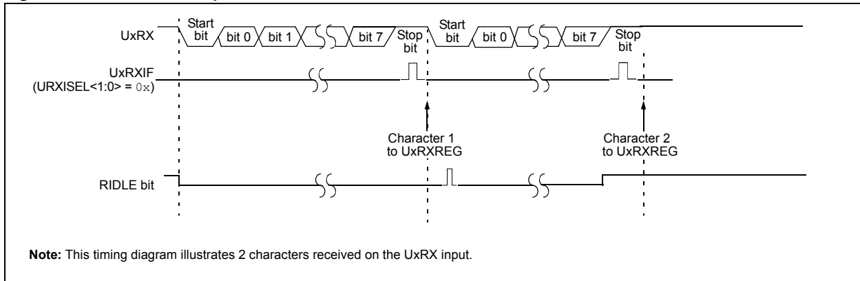
Figure 17-11: UART Reception
