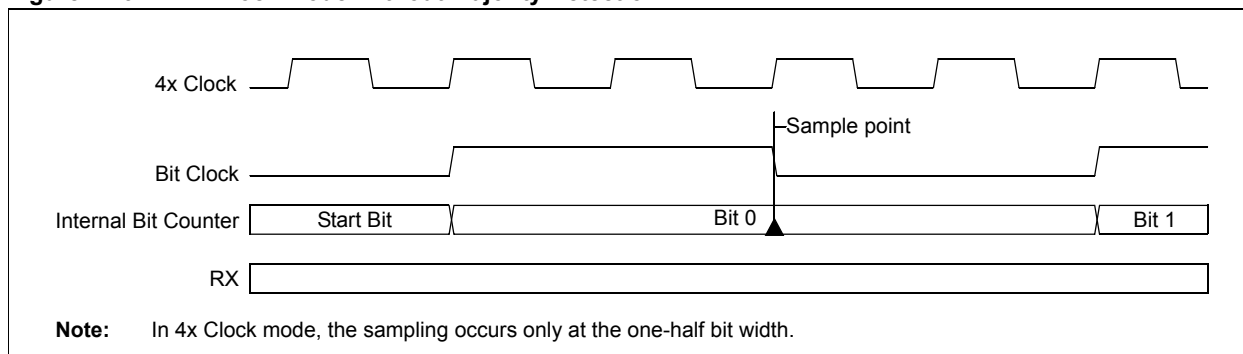
Figure 17-9: 4x Clock Mode Without Majority Detection
