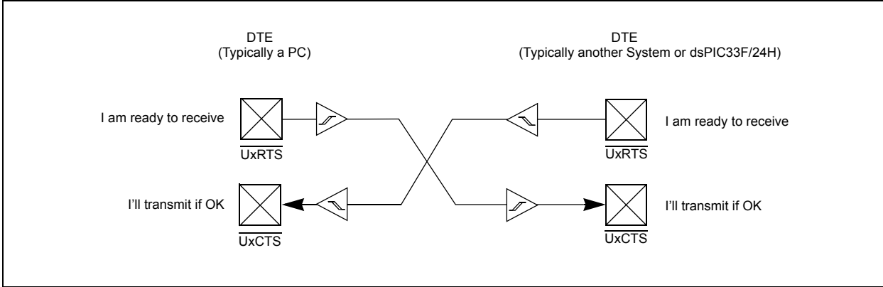
Figure 17-17: \overline{UxRTS}/\overline{UxCTS} Flow Control for DTE-DTE (RTSMD = 0, Flow Control Mode)
