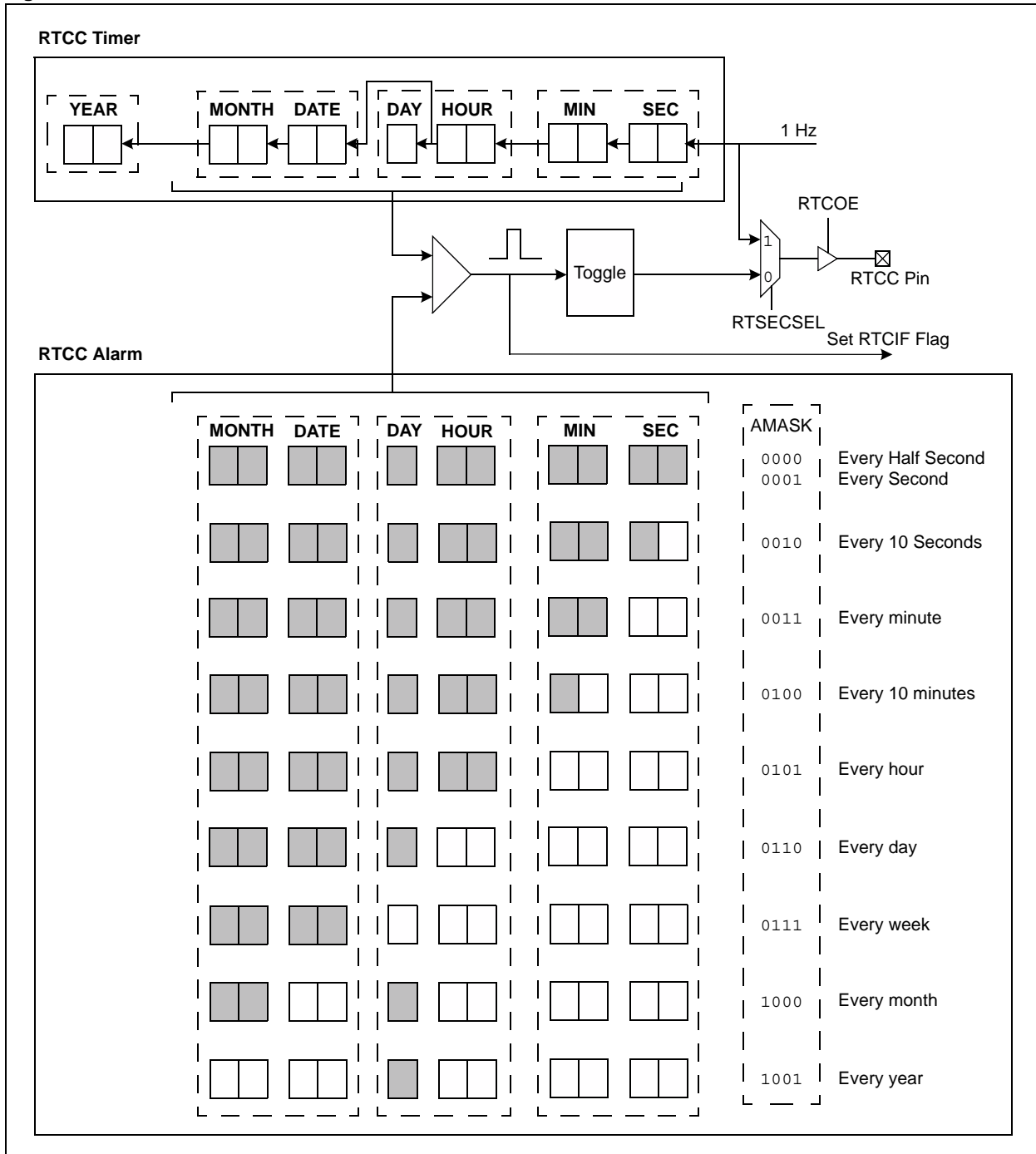
Figure 37-3: RTCC Alarm
