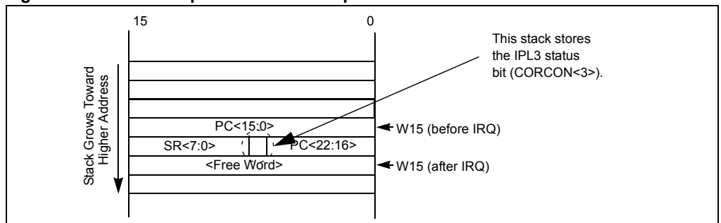
Figure 32-2: Stack Operation for Interrupt Event
