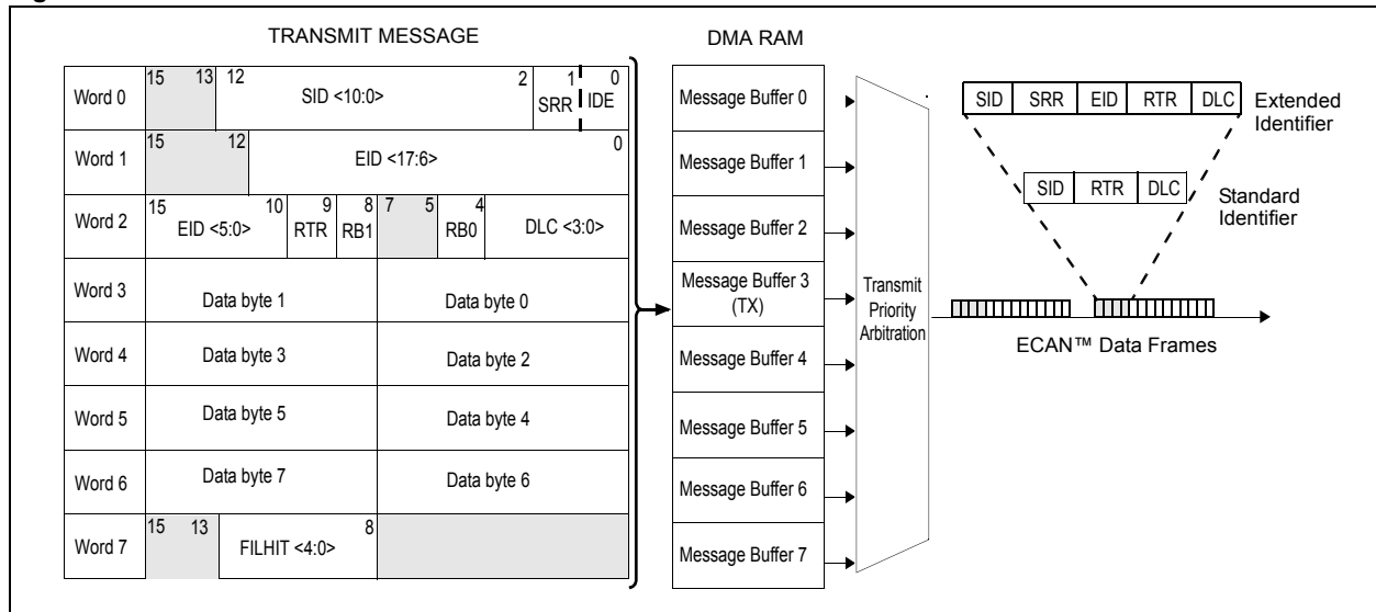
Figure 21-8: ECAN™ Transmission
