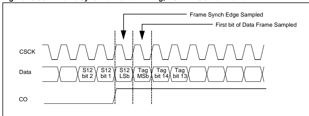
Figure 20-35: Frame Synchronization Timing, AC-Link Start of Frame
