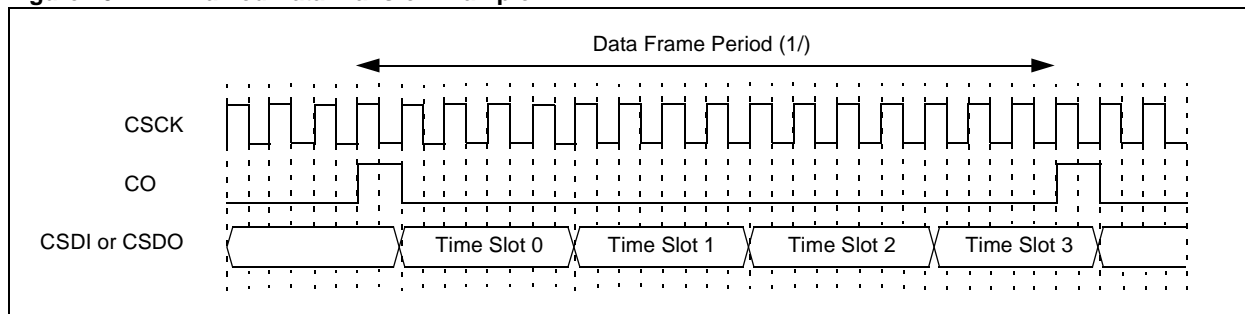
Figure 20-2: Framed Data Transfer Example
