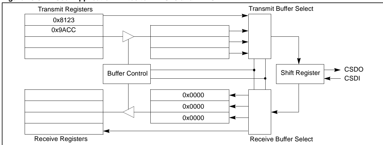
Figure 20-8: User Application Writes to TXBUF0 and TXBUF1
