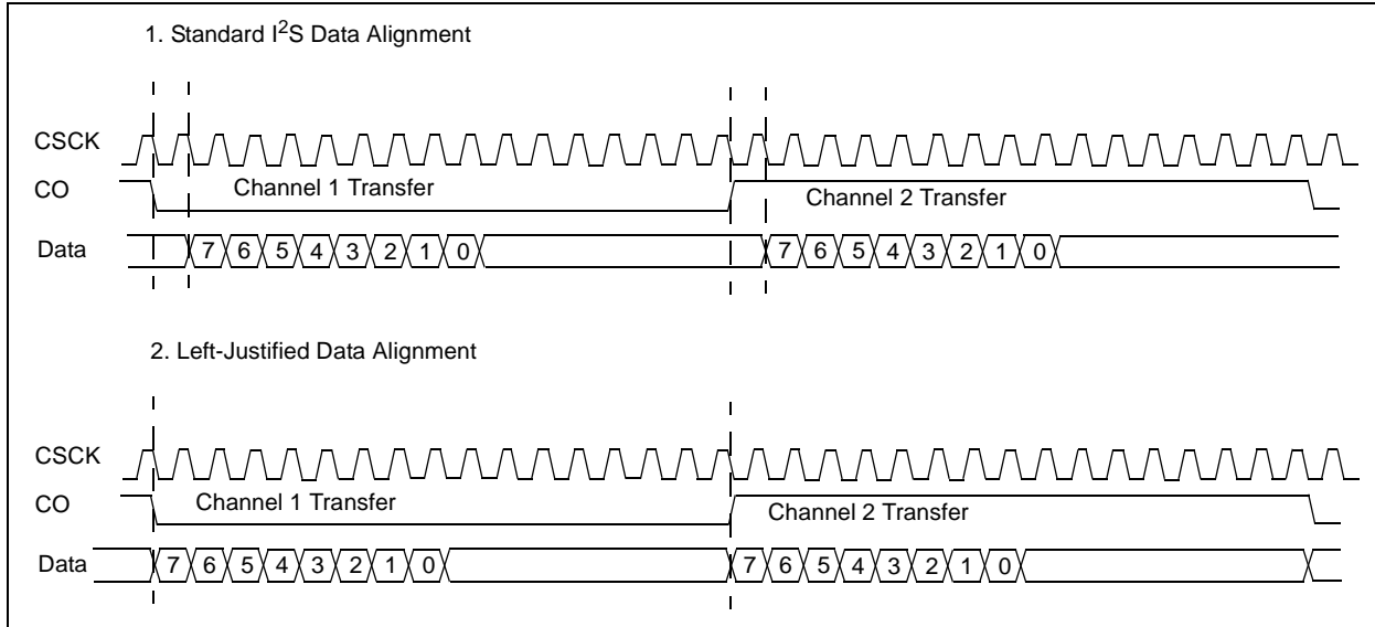
Figure 20-32: I 2 S Data Justification Options
