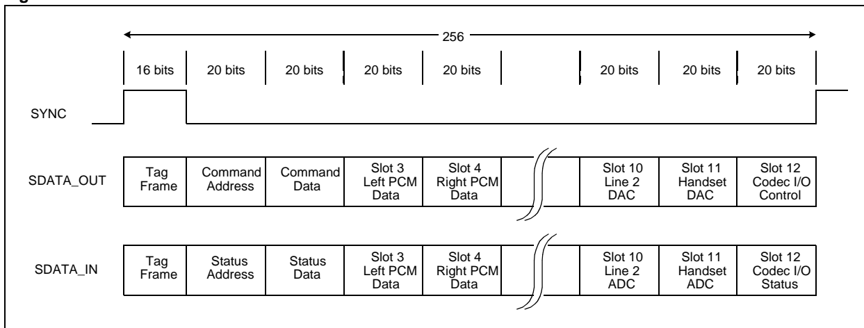
Figure 20-34: AC-Link Data Frame
