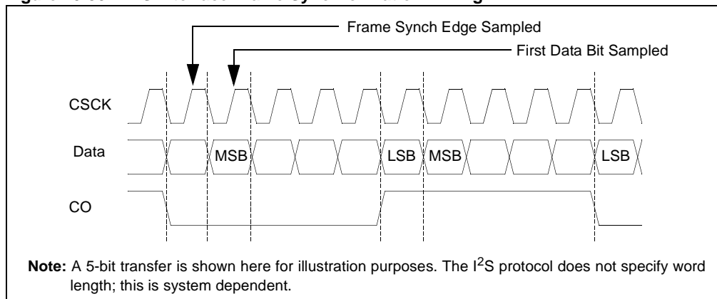
Figure 20-30: I 2 S Interface Frame Synchronization Timing
