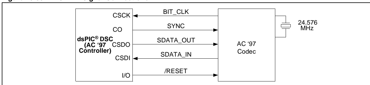
Figure 20-33: AC-Link Signal Connections
