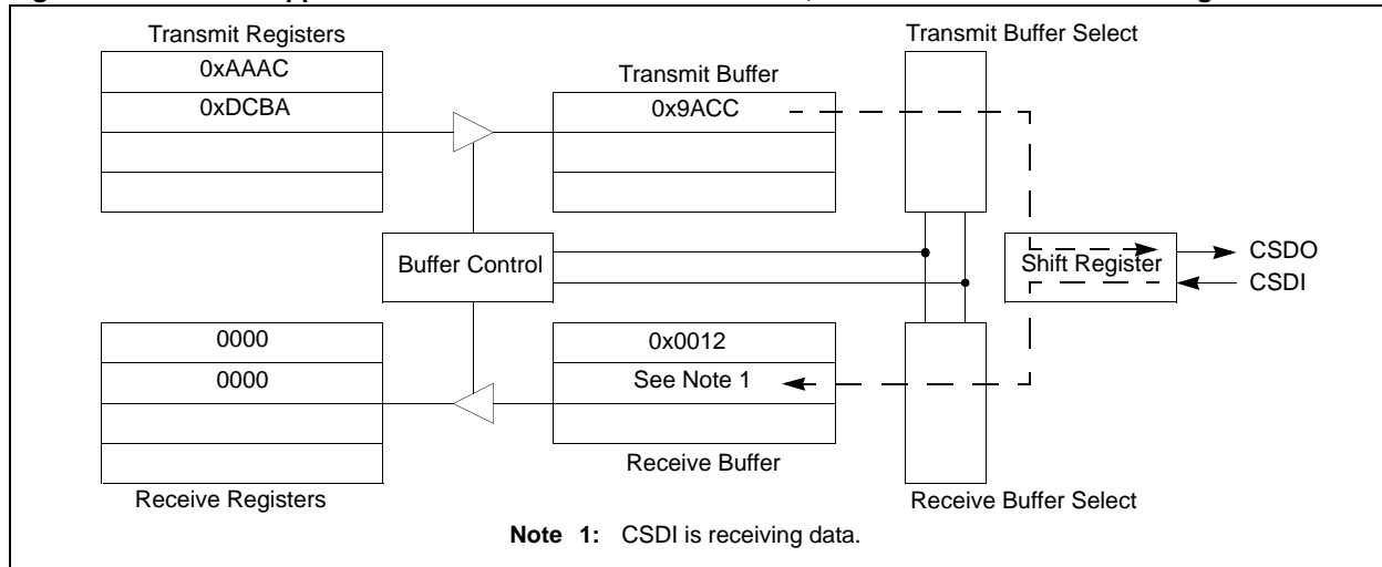
Figure 20-10: User Application Writes to TXBUF0 and TXBUF1, DCI Module Starts Transmitting Second Word
