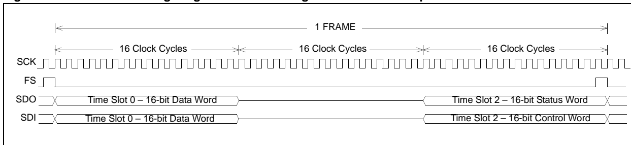
Figure 20-36: Codec Timing Diagram for DCI Configuration Code Example
