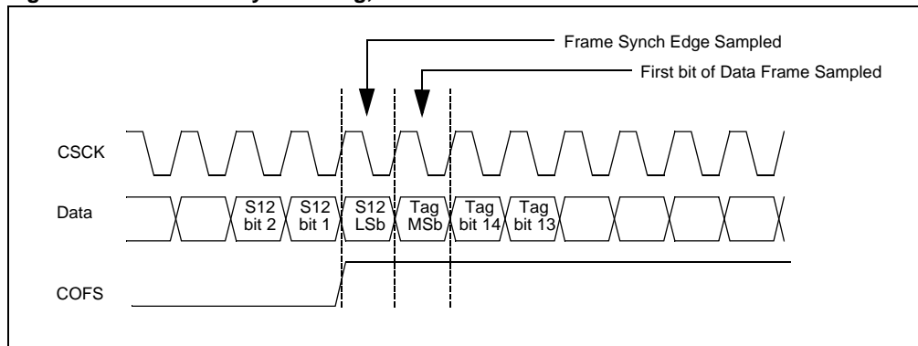
Figure 20-35: Frame Sync Timing, AC-Link Start of Frame
