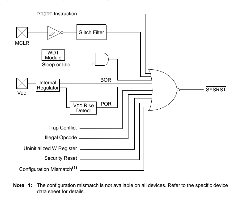
Figure 8-1: Reset System Block Diagram
