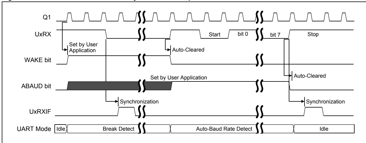
Figure 34-11: Break Detect Followed by Auto-Baud Sequence
