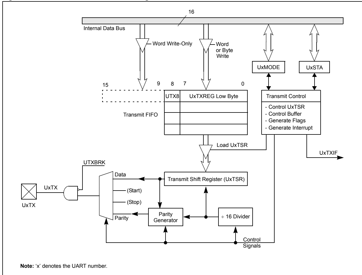
Figure 34-2: UART Transmitter Block Diagram
