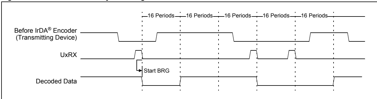
Figure 34-16: Inverted Polarity Decoding Results
