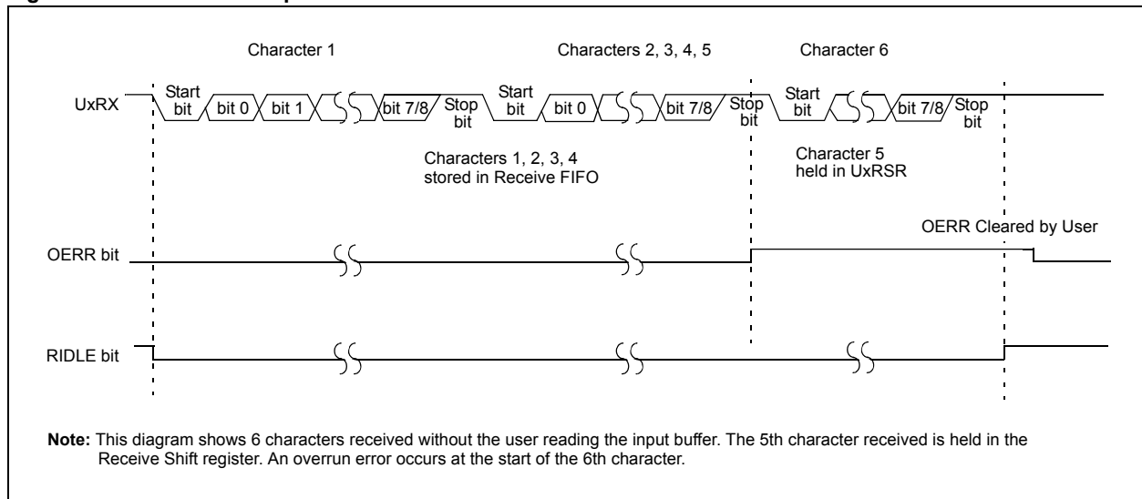
Figure 34-6: UART Reception with Receive Overrun
