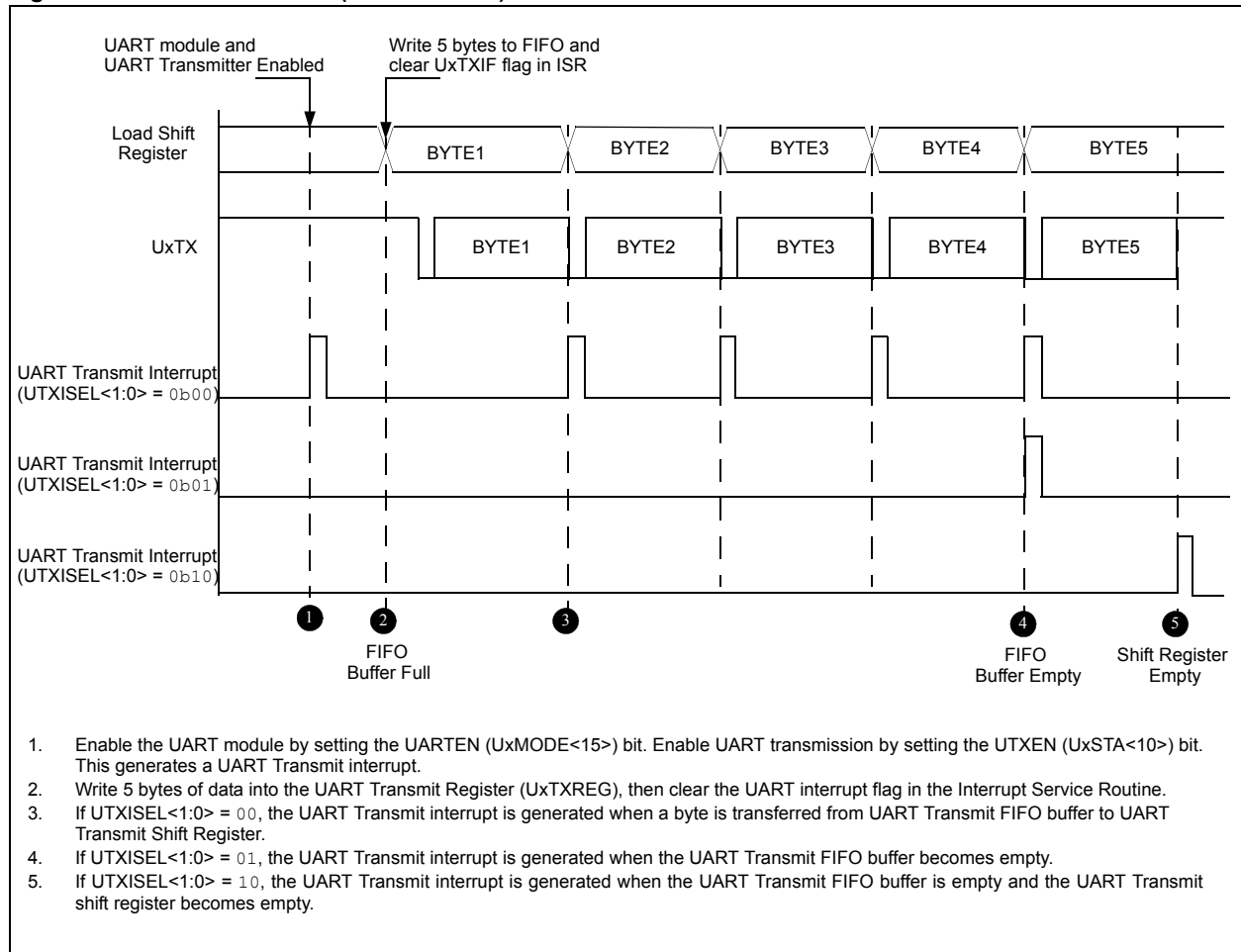
Figure 34-3: Transmission (Back-to-Back)
