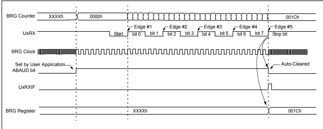
Figure 34-10: Automatic Baud Rate Calculation
