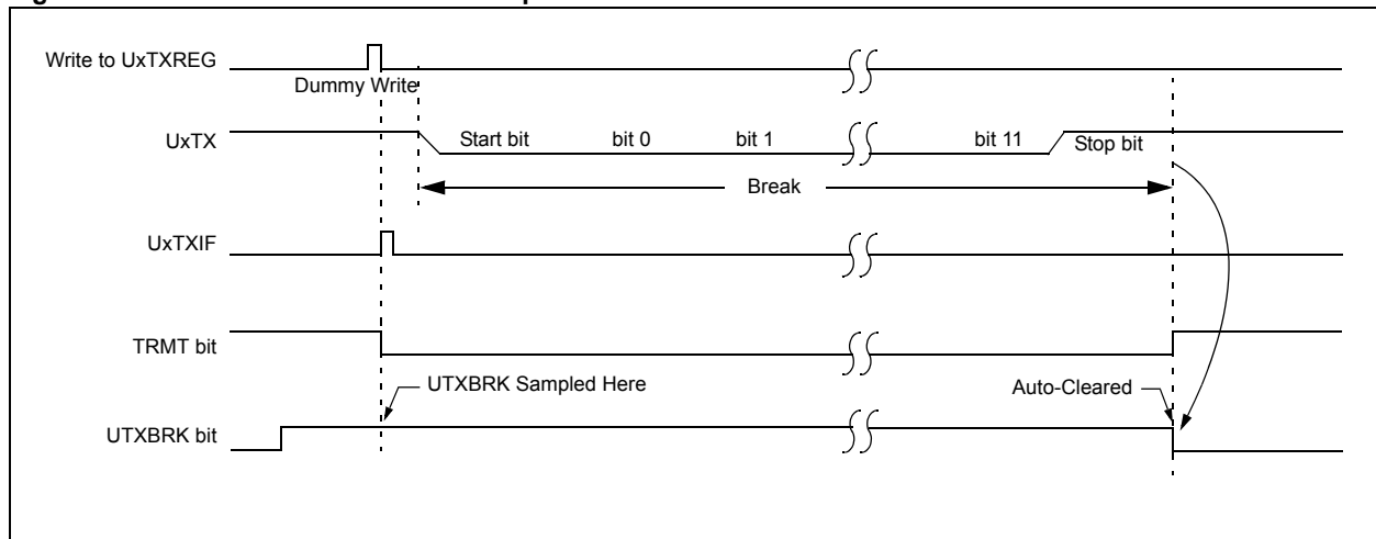
Figure 34-5: Send Break Character Sequence
