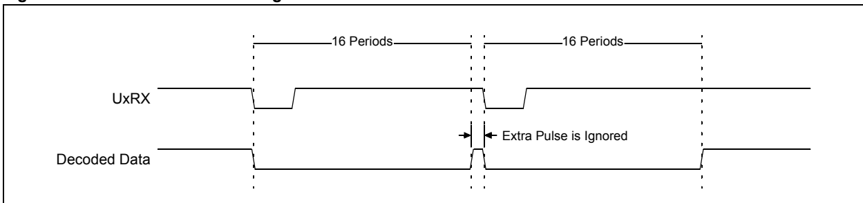
Figure 34-17: Clock Jitter Causing a Pulse Between Consecutive Zeros
