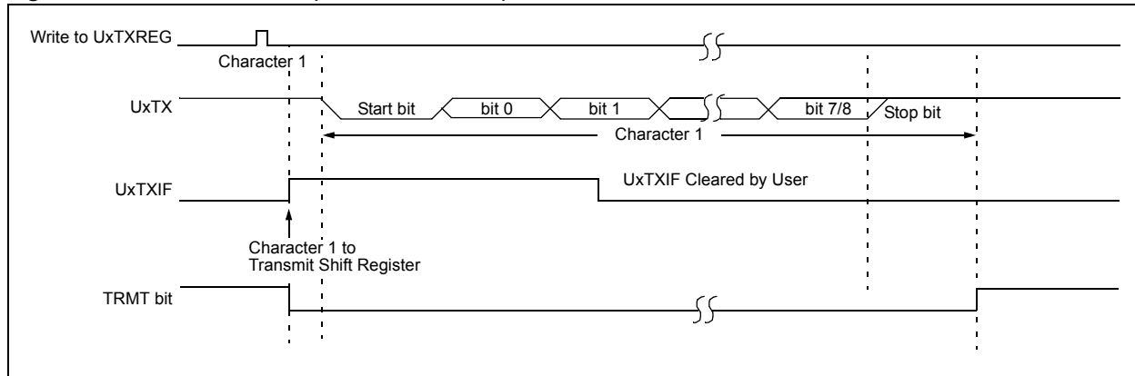
Figure 34-4: Transmission (8-Bit or 9-Bit Data)
