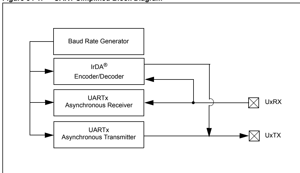
Figure 34-1: UART Simplified Block Diagram
