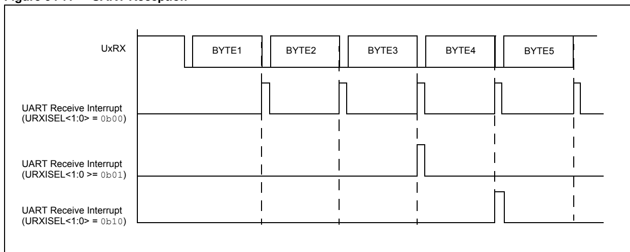
Figure 34-7: UART Reception
