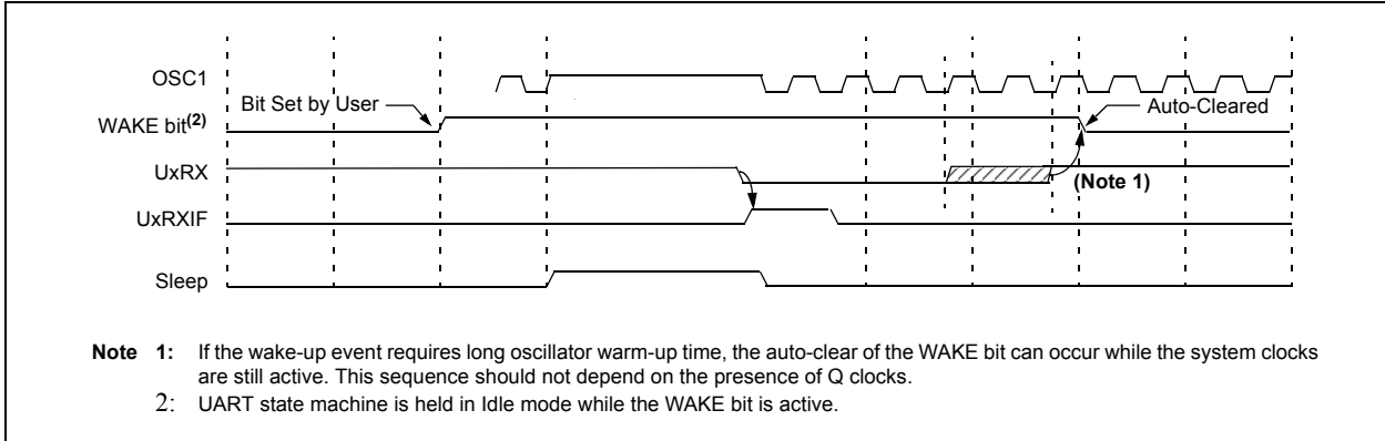
Figure 34-19: Auto-Wake-up Bit (WAKE) Timings During Sleep
