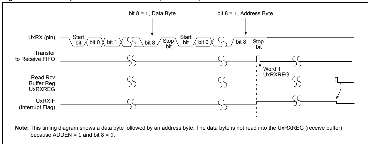
Figure 34-9: Reception with Address Detect (ADDEN = 1)
