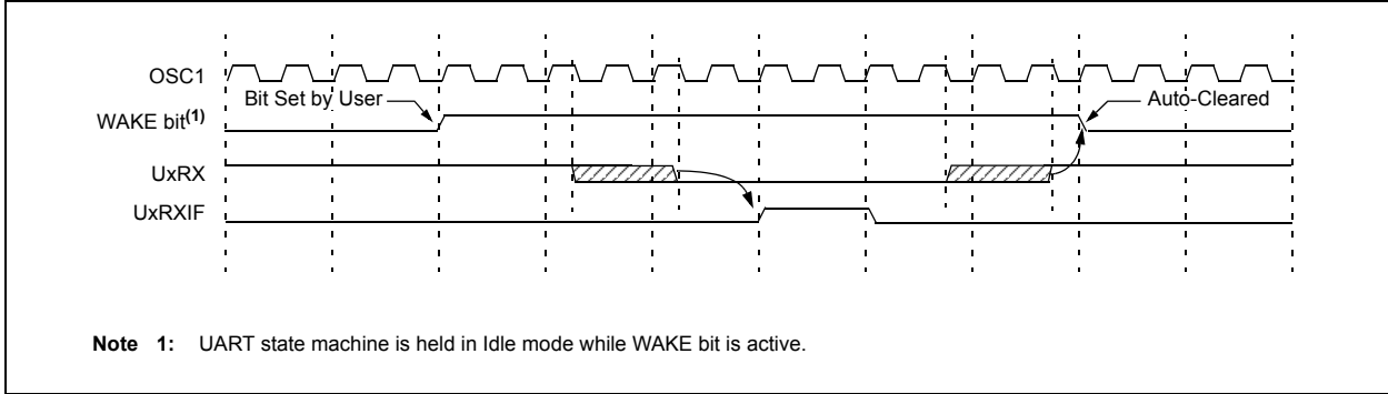
Figure 34-18: Auto-Wake-up Bit (WAKE) Timings During Normal Operation
