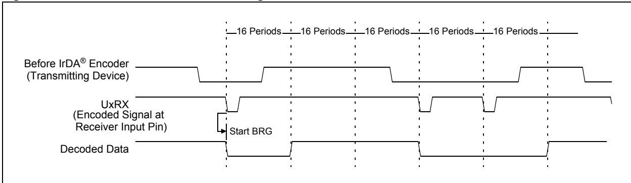
Figure 34-15: Macro View of IrDA® Decoding Scheme
