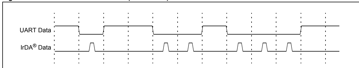
Figure 34-13: IrDA® Encode Scheme (UTxINV = 0)
