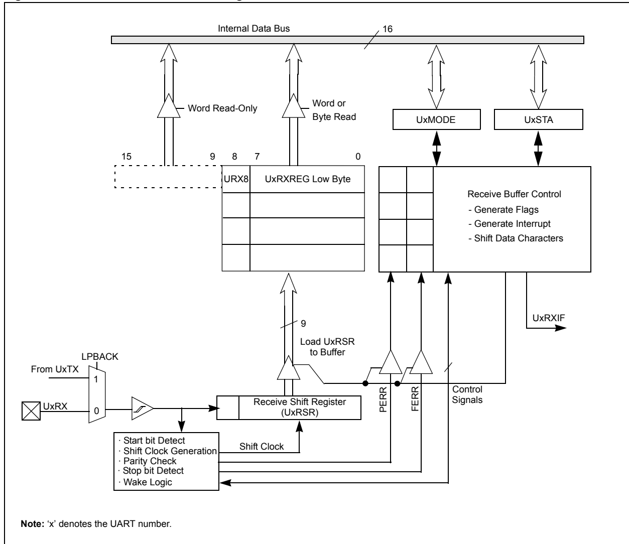
Figure 34-8: UART Receiver Block Diagram
