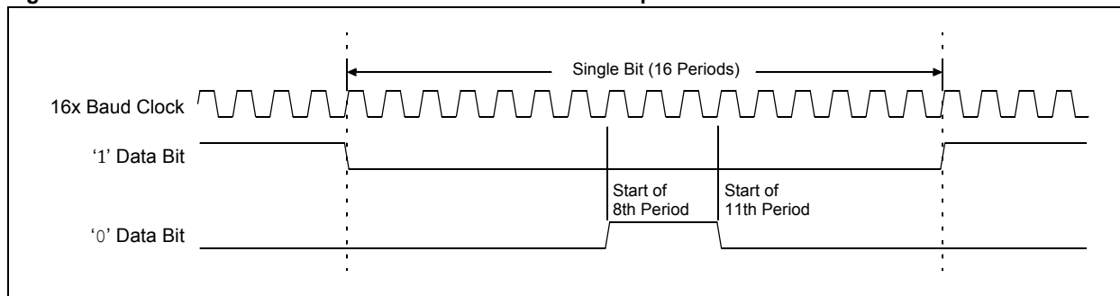
Figure 34-12: IrDA® Encode Scheme for '0' Bit Data with Respect to 16x Baud Clock
