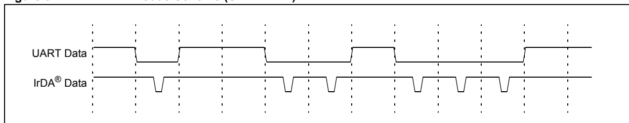
Figure 34-14: IrDA® Encode Scheme (UTxINV = 1)
