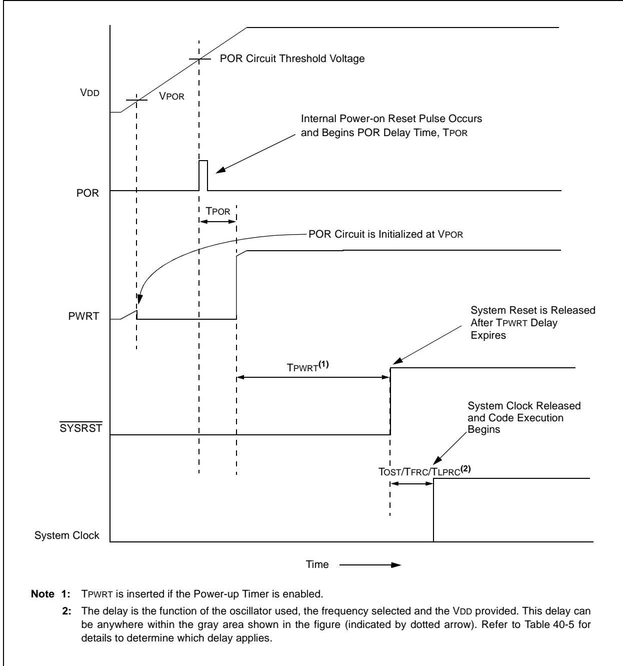
Figure 40-2: POR Module Timing Sequence for Rising VDD
