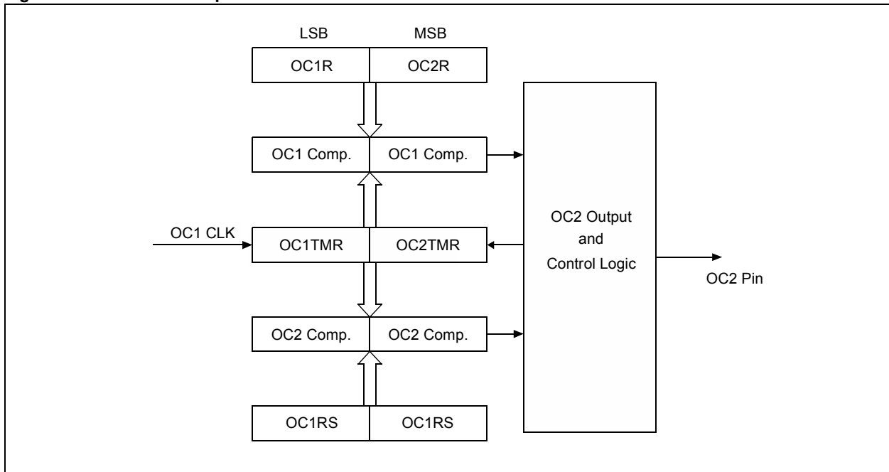
Figure 35-26: Cascade Operation
